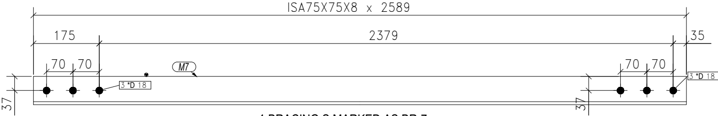
4-BRACING S MARKED AS BR-7
