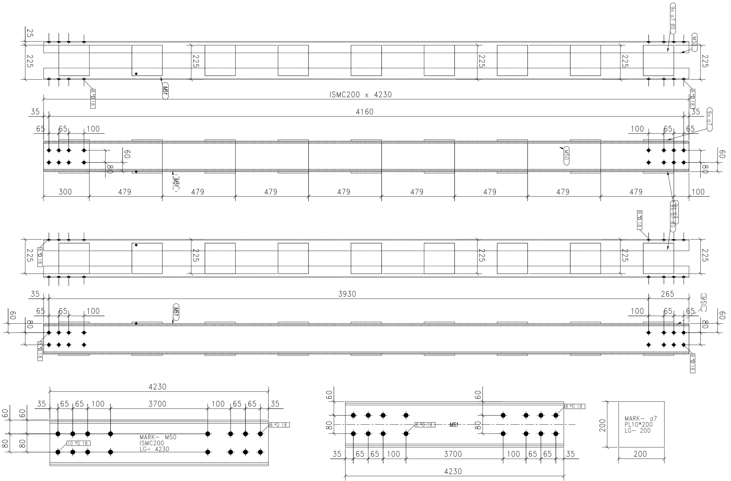
4-VERTICAL BRACES MARKED AS V-1
