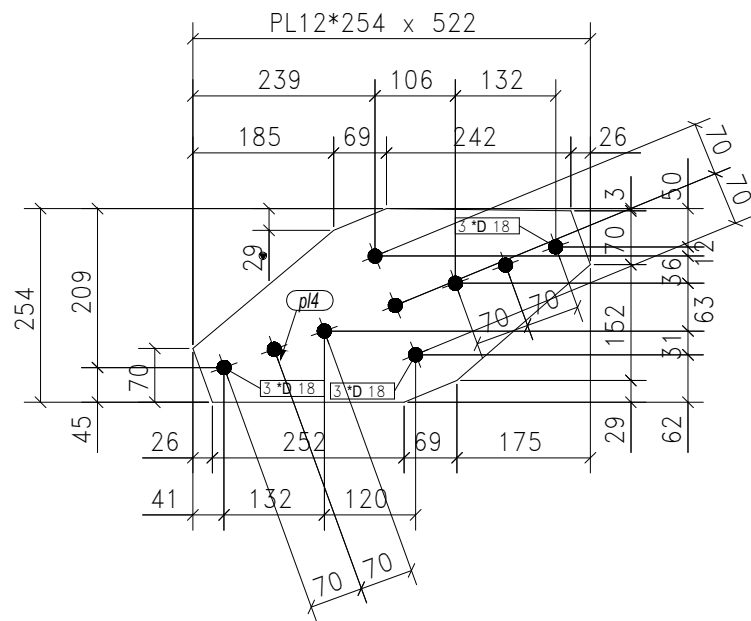
2-GUSSET PLATES MARKED AS G8
