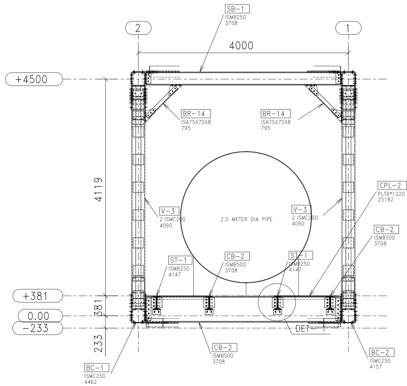
SECTION OF BRIDGE AT GRID A AND G
