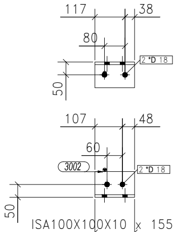
48-ANGLES MARKED AS CA-2
