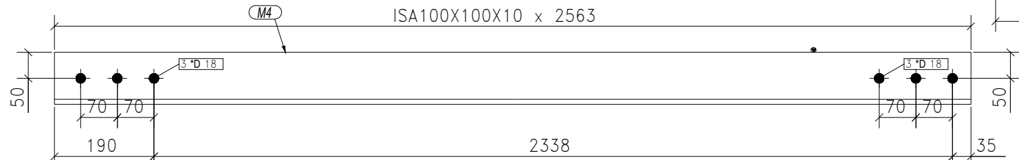
ONE-BRACING MARKED AS BR-4
