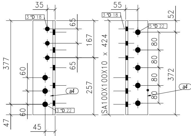
12-CLIP ANGLES MARKED AS CA-6
