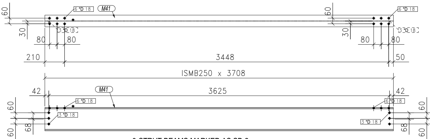
3-STRUT BEAMS MARKED AS SB-2
