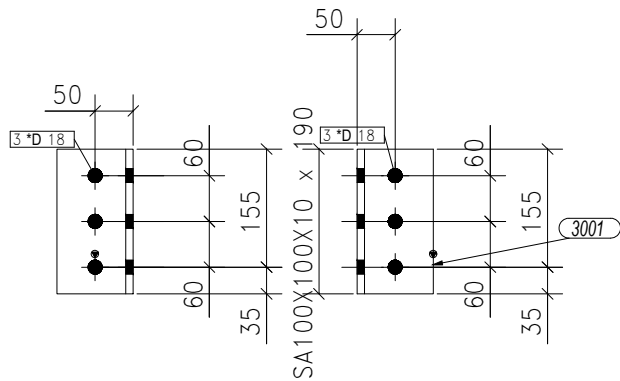
96-ANGLES MARKED AS CA-1
