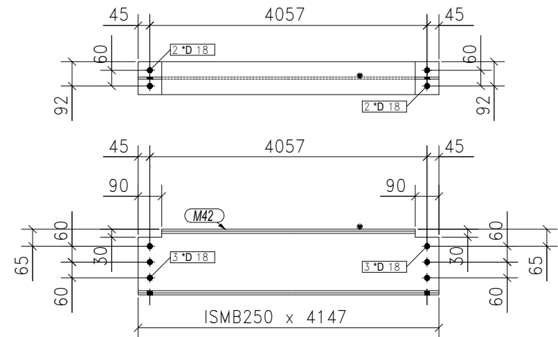
24-STRINGER BEAMS MARKED AS ST
