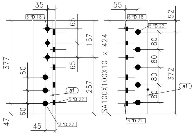
2-CLIP ANGLES MARKED AS CA-3
