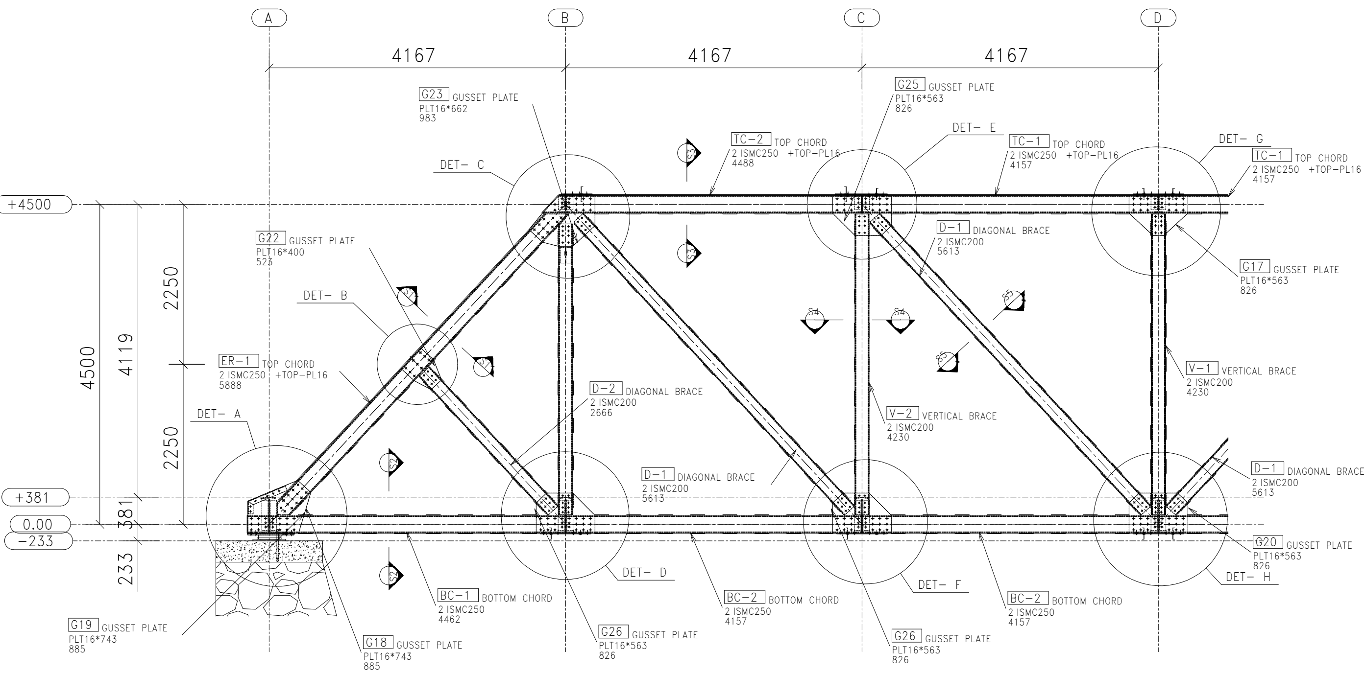
ELEVATION OF BRIDGE (MIRROR HALF SPAN )
