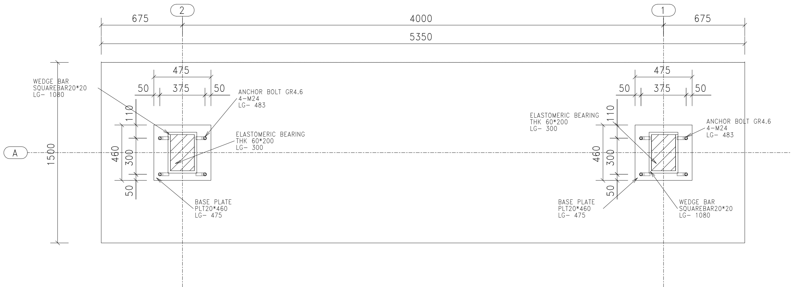
TYP. BEARING PLAN TOP VIEW
