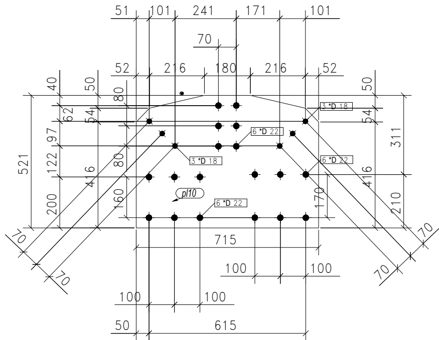
8-GUSSET PLATES MARKED AS G13
