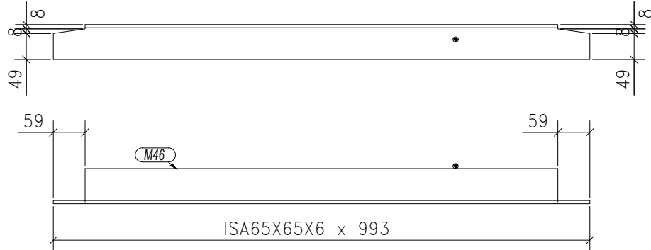
60-CHQPL RIBS MARKED AS CPL-1
