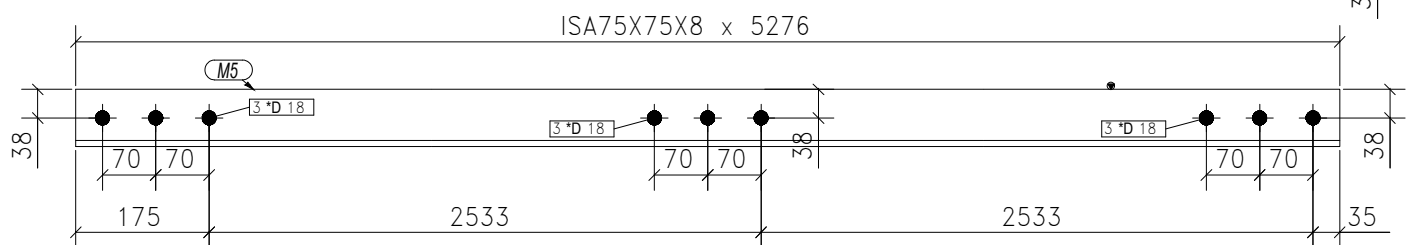
16-BRACING S MARKED AS BR-5
