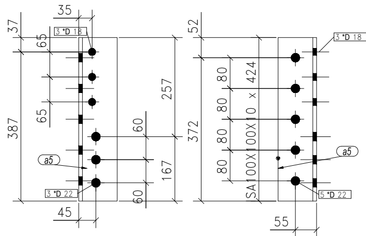
12-CLIP ANGLES MARKED AS CA-7
