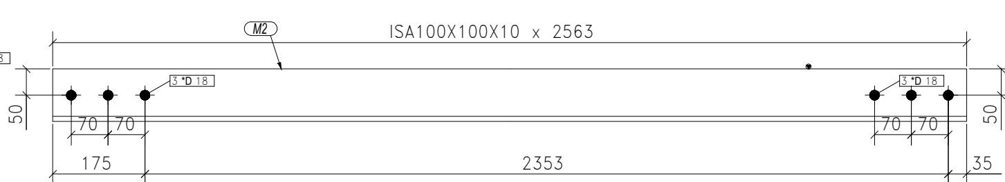
4-BRACING S MARKED AS BR-2
