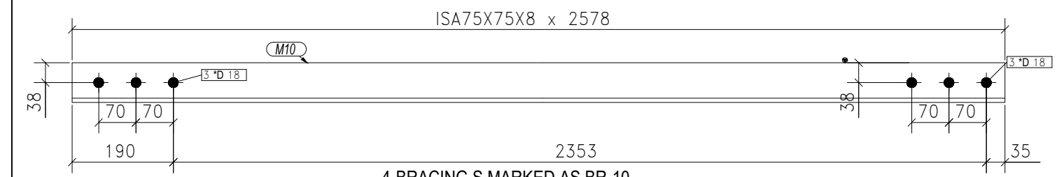
4-BRACING S MARKED AS BR-10
