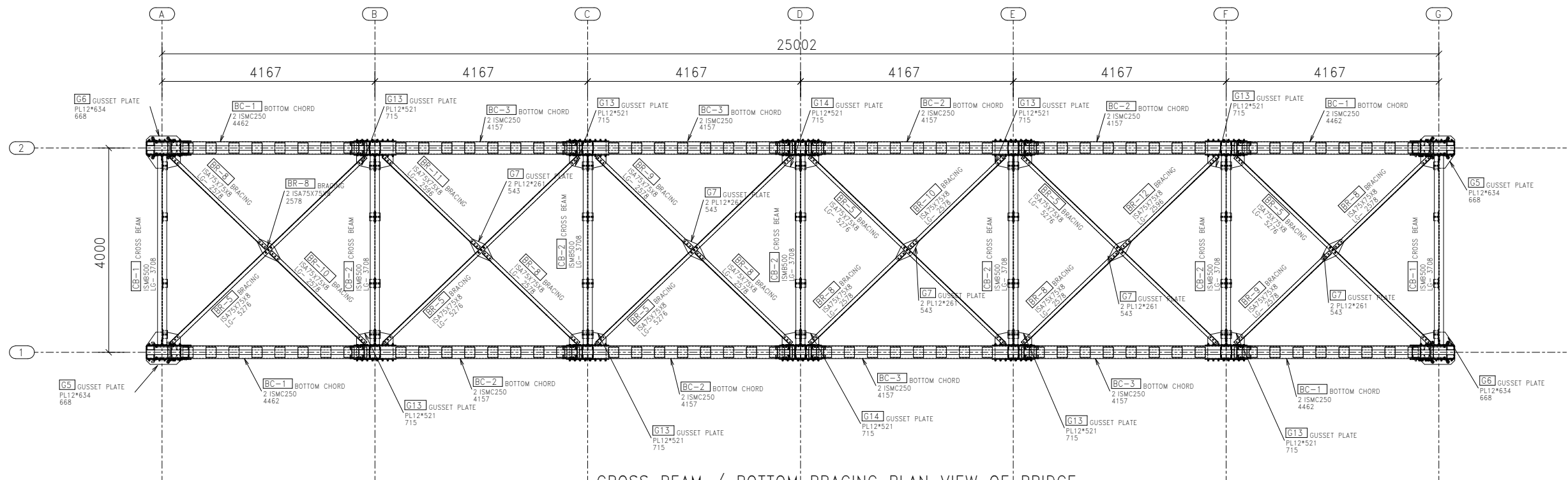
CROSS BEAM / BOTTOM BRACING PLAN VIEW OF BRIDGE
