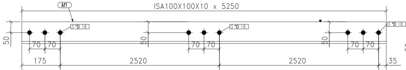
4-BRACING S MARKED AS BR-1
