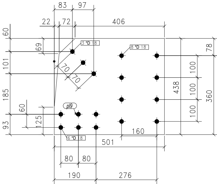
4-GUSSET PLATES MARKED AS G12
