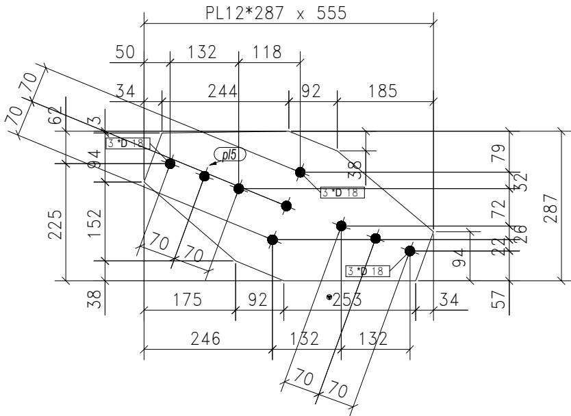
2-GUSSET PLATES MARKED AS G9
