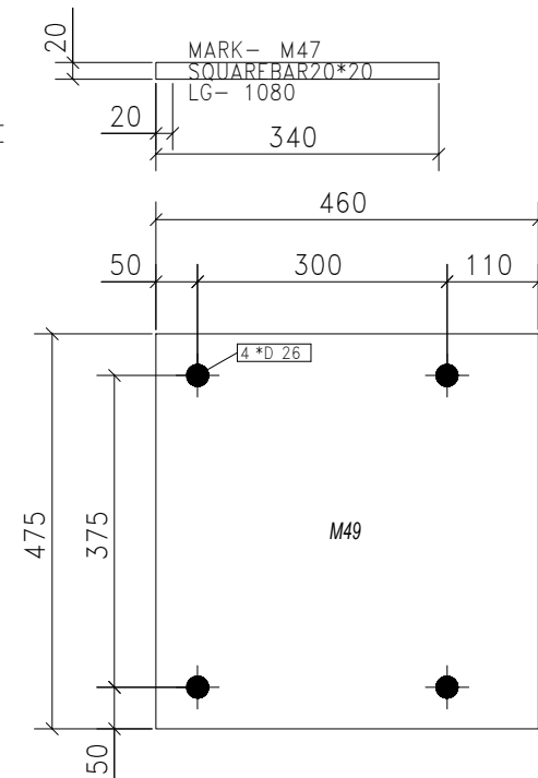
2-BASE PLATES MARKED AS BP-1
