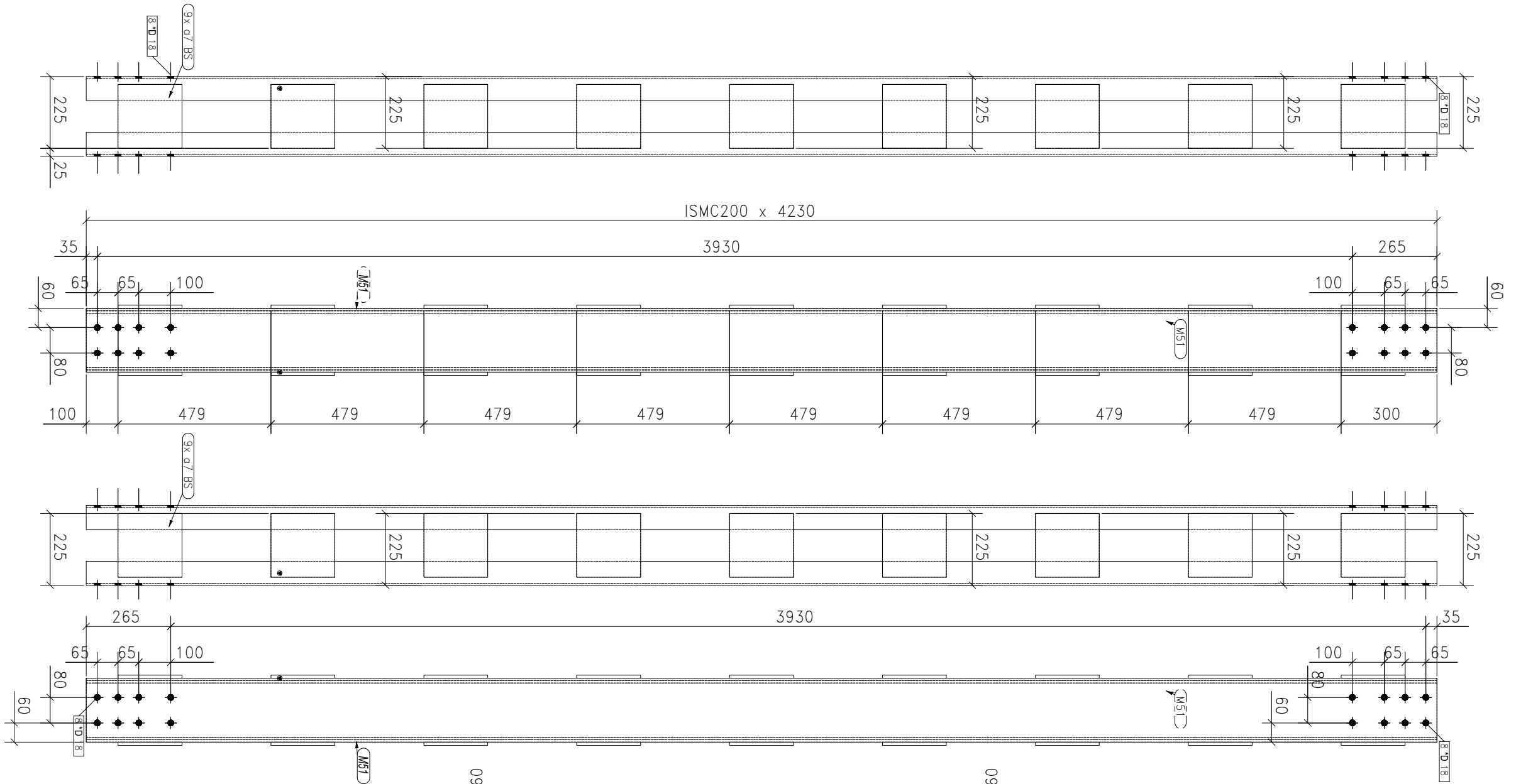
4-VERTICAL BRACES MARKED AS V-2
