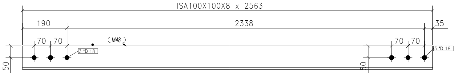
ONE-BRACING MARKED AS BR-15
