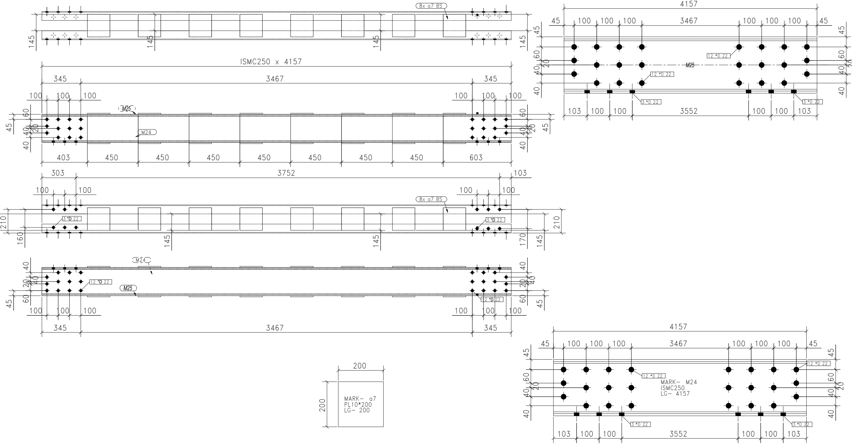
4-BOTTOM CHORDS MARKED AS BC-2
