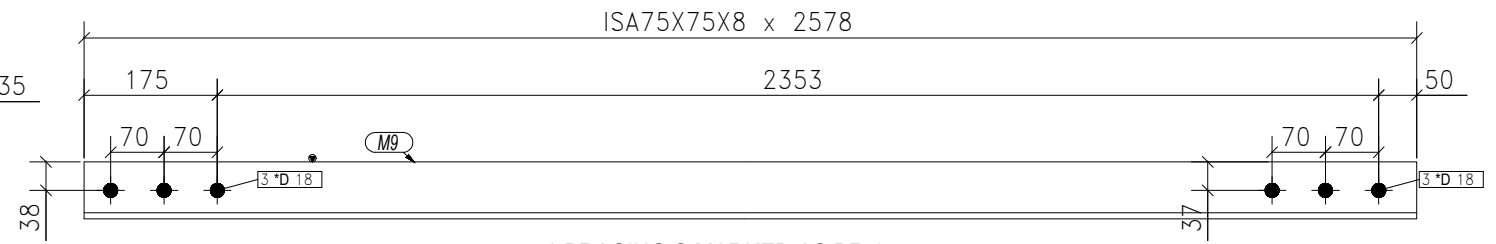
4-BRACING S MARKED AS BR-9
