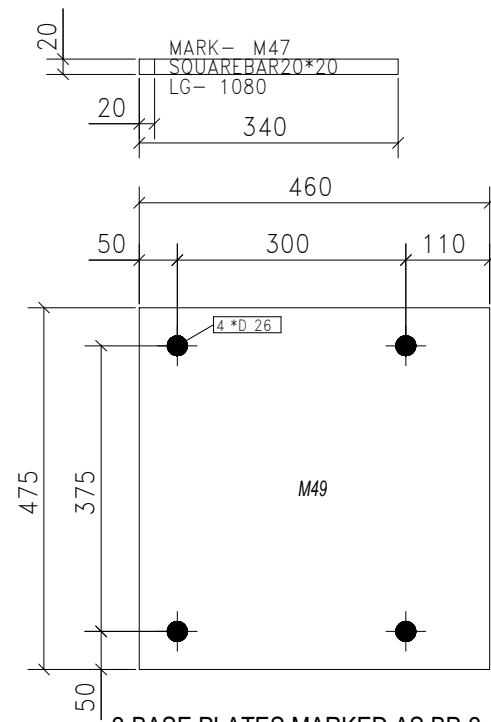
2-BASE PLATES MARKED AS BP-2
