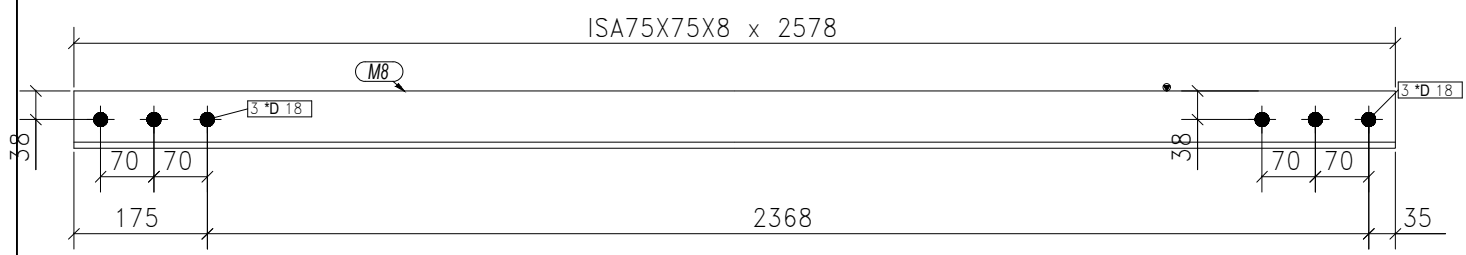
12-BRACING S MARKED AS BR-8
