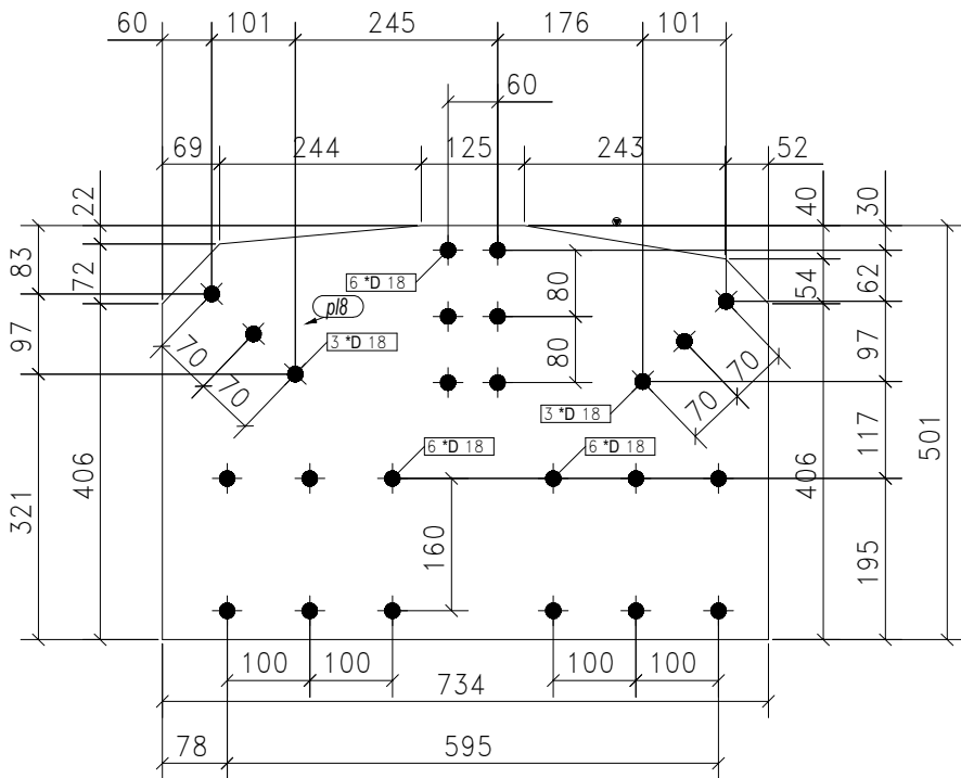
4-GUSSET PLATES MARKED AS G11
