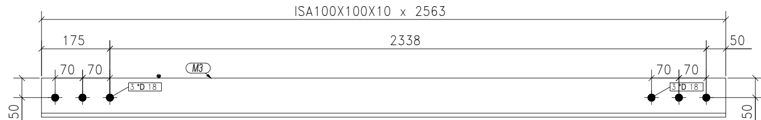
2-BRACING S MARKED AS BR-3
