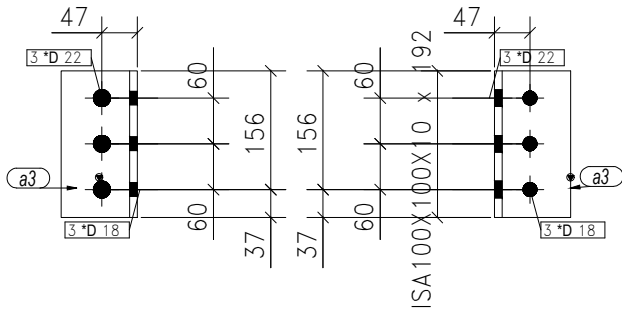
20-CLIP ANGLES MARKED AS CA-5
