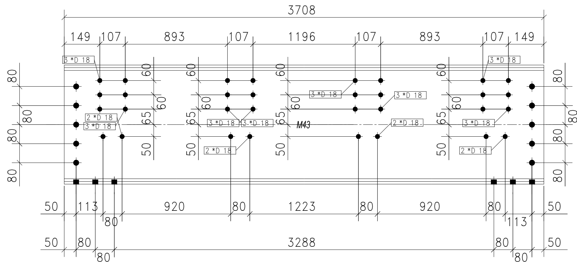
2-CROSS BEAMS MARKED AS CB-1
