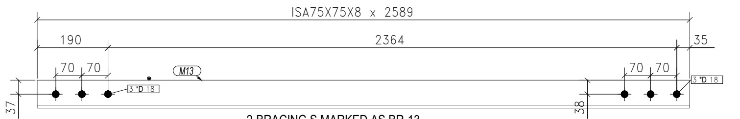
2-BRACING S MARKED AS BR-13
