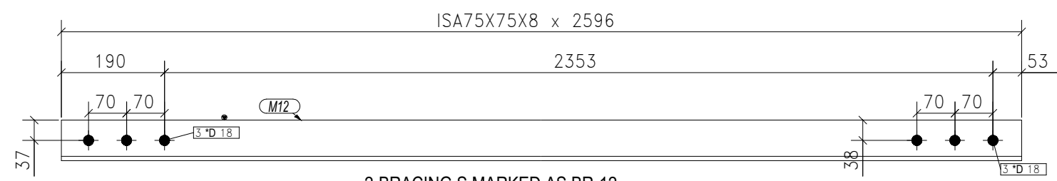
2-BRACING S MARKED AS BR-12
