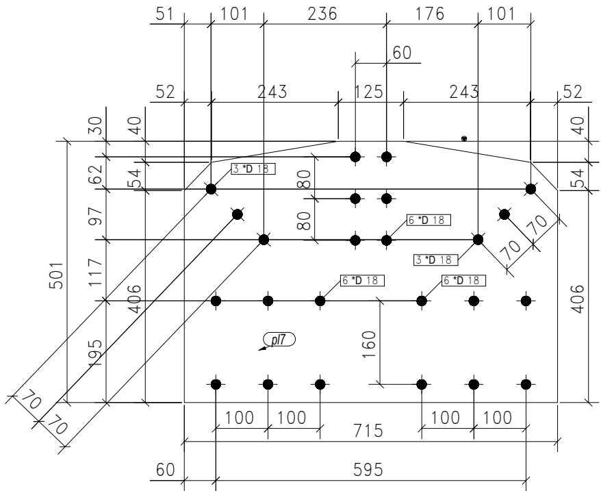
2-GUSSET PLATES MARKED AS G10
