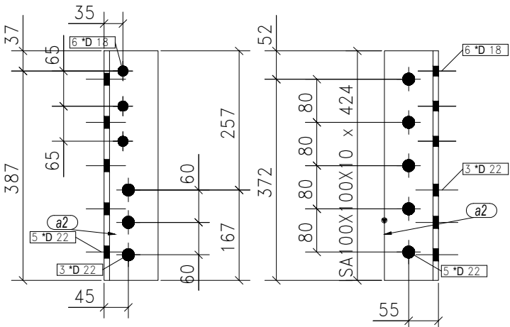
2-CLIP ANGLES MARKED AS CA-4
