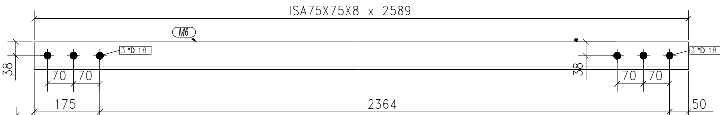
2-BRACING S MARKED AS BR-6
