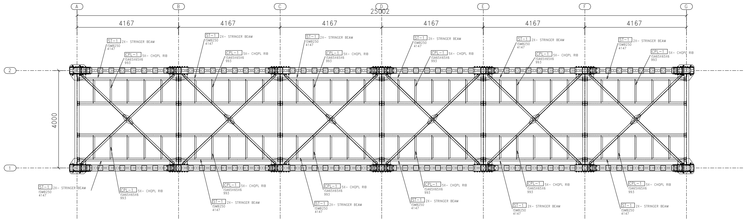
STRINGER PLAN VIEW OF BRIDGE
