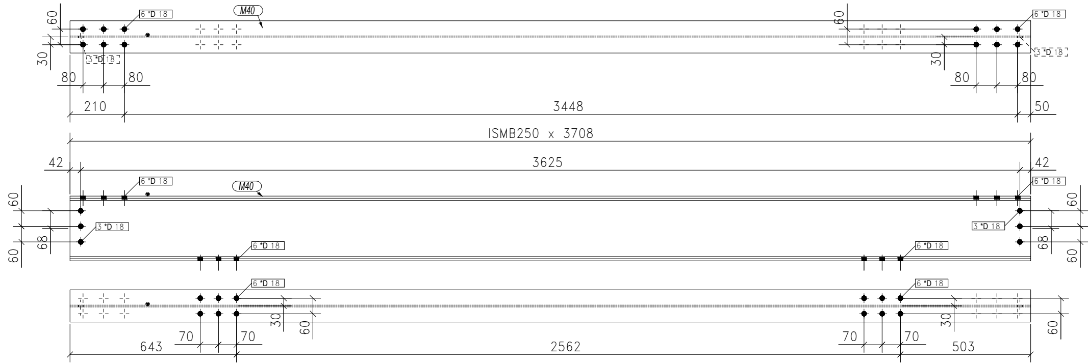
2-STRUT BEAMS MARKED AS SB-1
